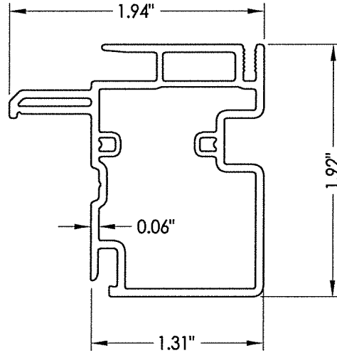
6 MEETING STILE
