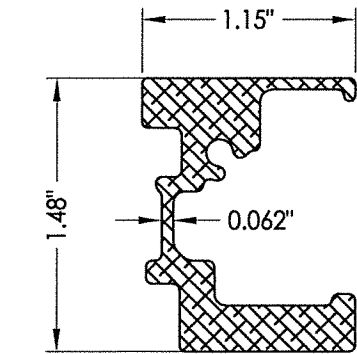
9 MEETING STILE REINFORCEMENT
