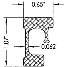
19 FLORIDA FLANGE (Optional)
