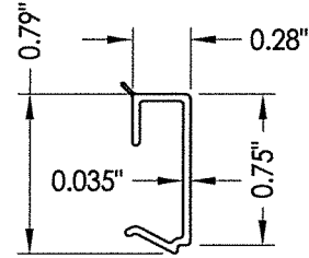
2 GLAZING BEAD
