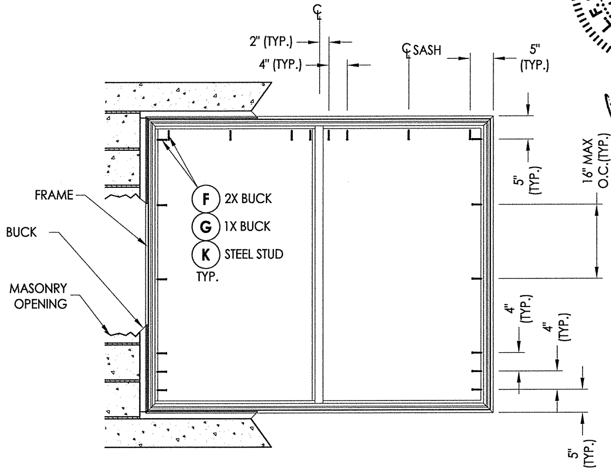
FRAME ANCHORING
